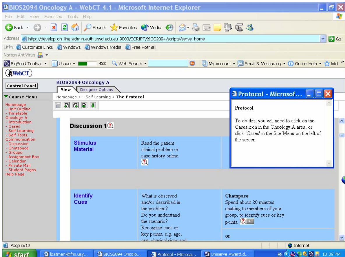
Figure 1. Screen of the step-by-step explanation of Discussion 1 in the Protocol, showing the use of text based hints (inset) and audio hints, represented by a question mark and play button, respectively 1
